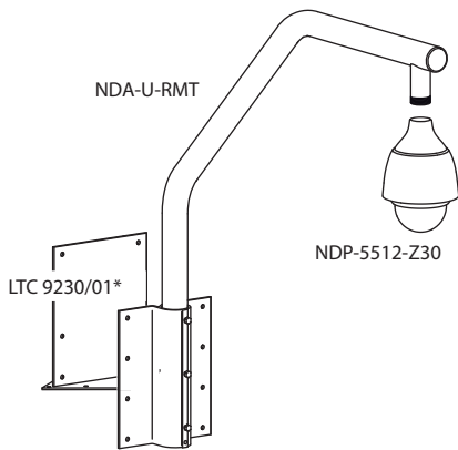
Roof mount (IP66) * optional for flat roof mount
